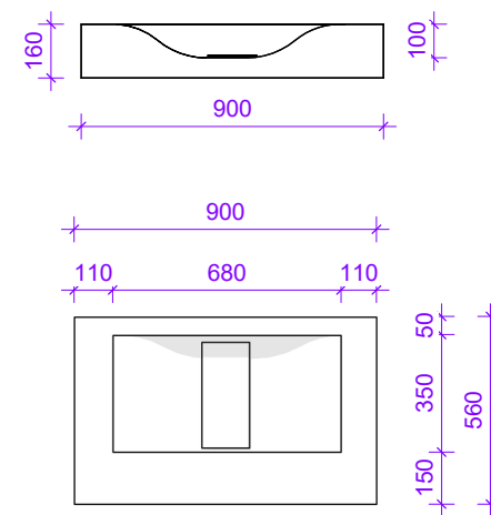
Plan Detail
