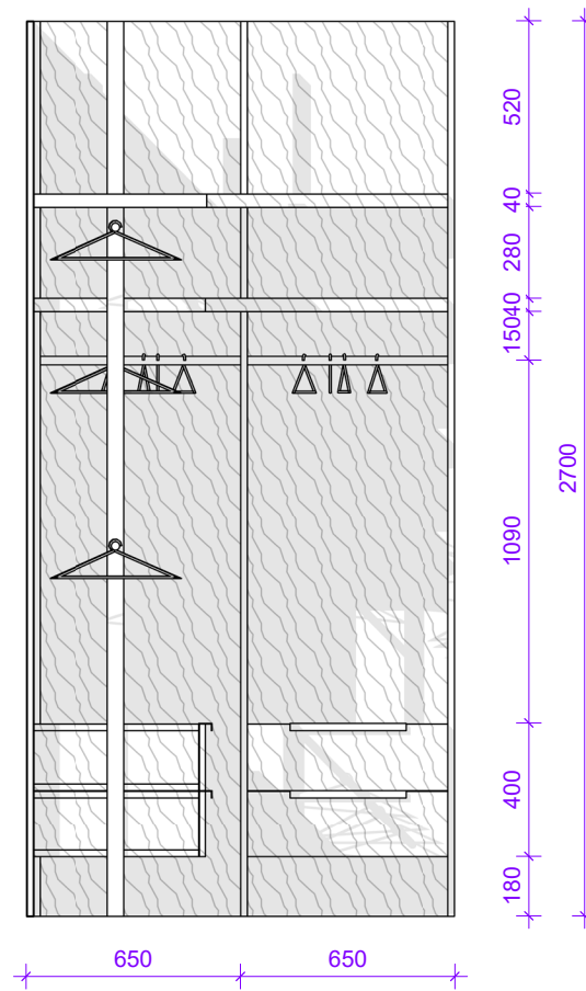
Elevation Front 1 : 25
