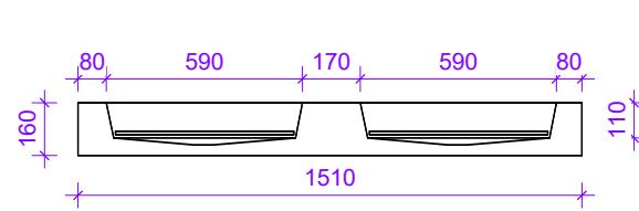
Elevation Left
