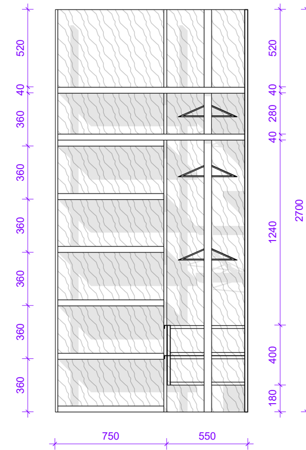
Elevation Back 1 : 25
